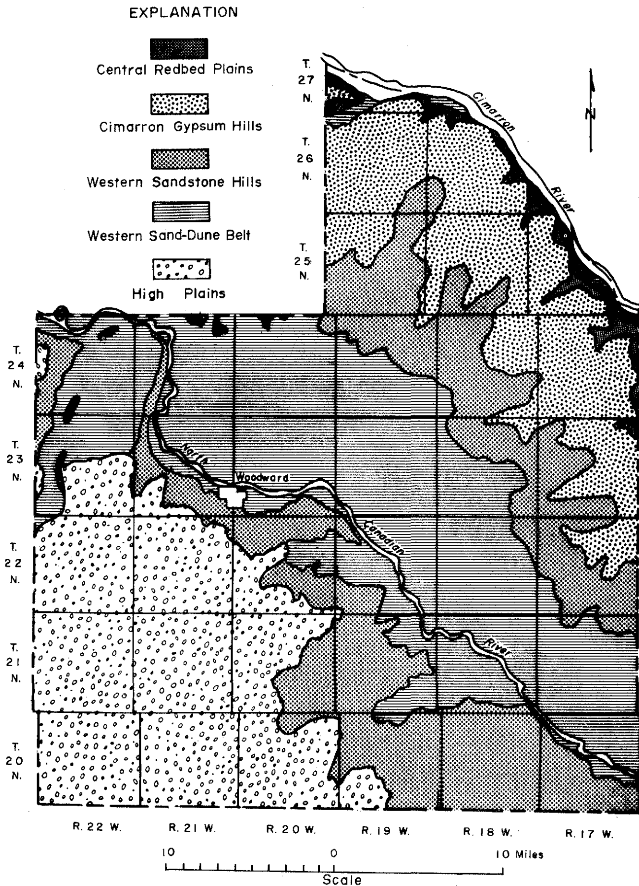
FIG. 3-- MAP OF WOODWARD COUNTY, OKLAHOMA, SHOWING GEOMORPHIC UNITS (Modified after Curtis and Ham, 1957)
