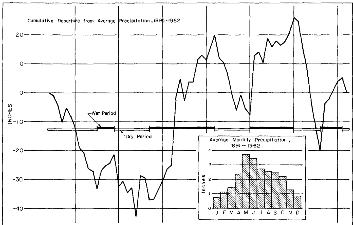
FIG. 4-- GRAPHS SHOWING PRECIPITATION AT WOODWARD , OKLAHOMA
