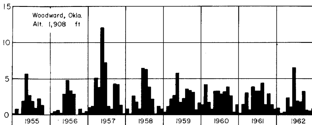
FIG. 5 -- GRAPHS SHOWING WATER-LEVEL FLUCTUATIONS IN REPRESENTATIVE WELLS TAPPING THE OGALLALA FORMATION AND THE HIGH-TERRACE DEPOSITS; AND PRECIPITATION AT WOODWARD
