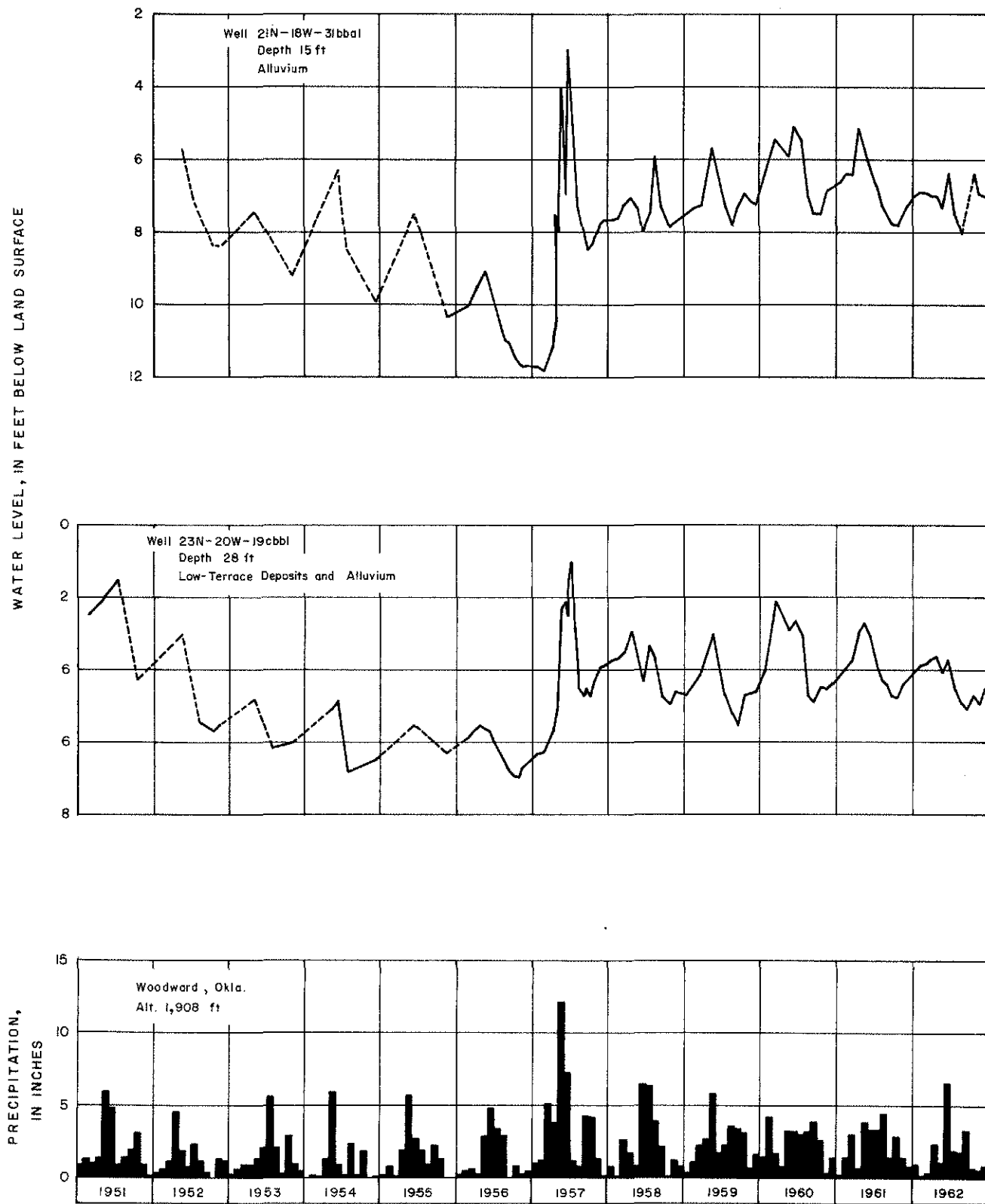
FIG. 6-- GRAPHS SHOWING WATER-LEVEL FLUCTUATIONS IN REPRESENTATIVE WELLS TAPPING THE LOW-TERRACE DEPOSITS AND ALLUVIUM; AND PRECIPITATION AT WOODWARD
