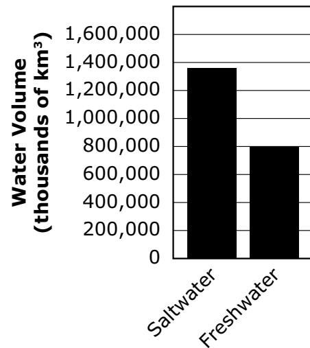
Earth's Total Saltwater and Freshwater Sources
