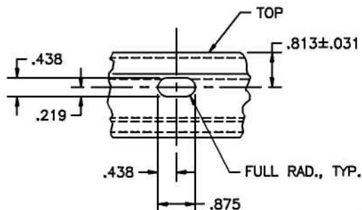
TYPICAL SLOTTED HOLE DETAIL
