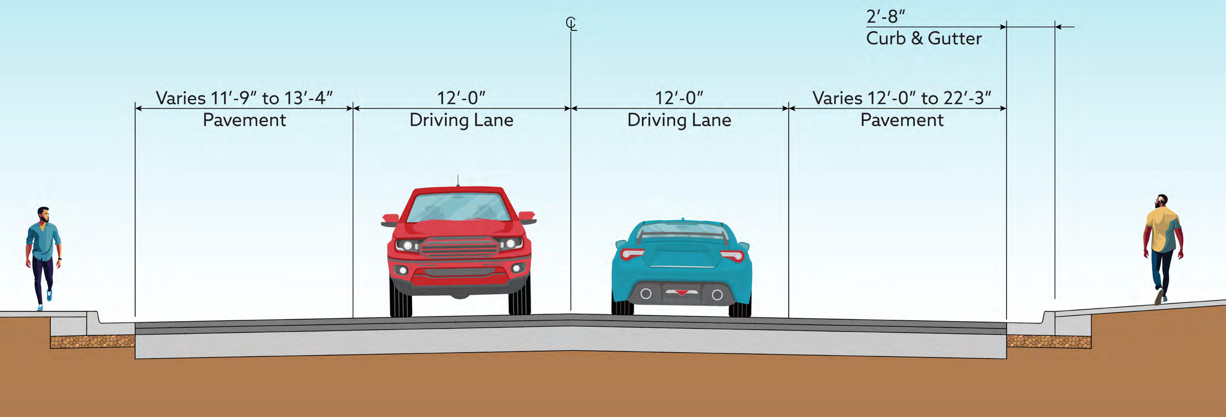
US-64 Roadway Widening From SH-104 (Franklin Street) to First Assembly Church of God
