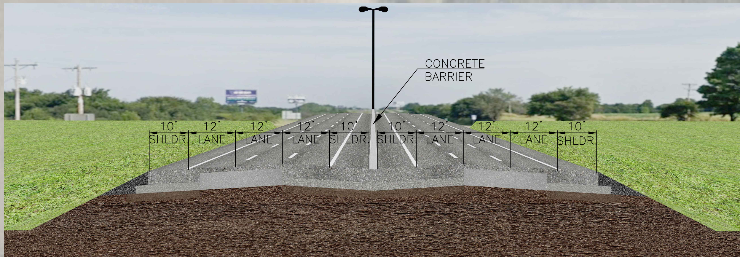
MAINLINE TYPICAL
