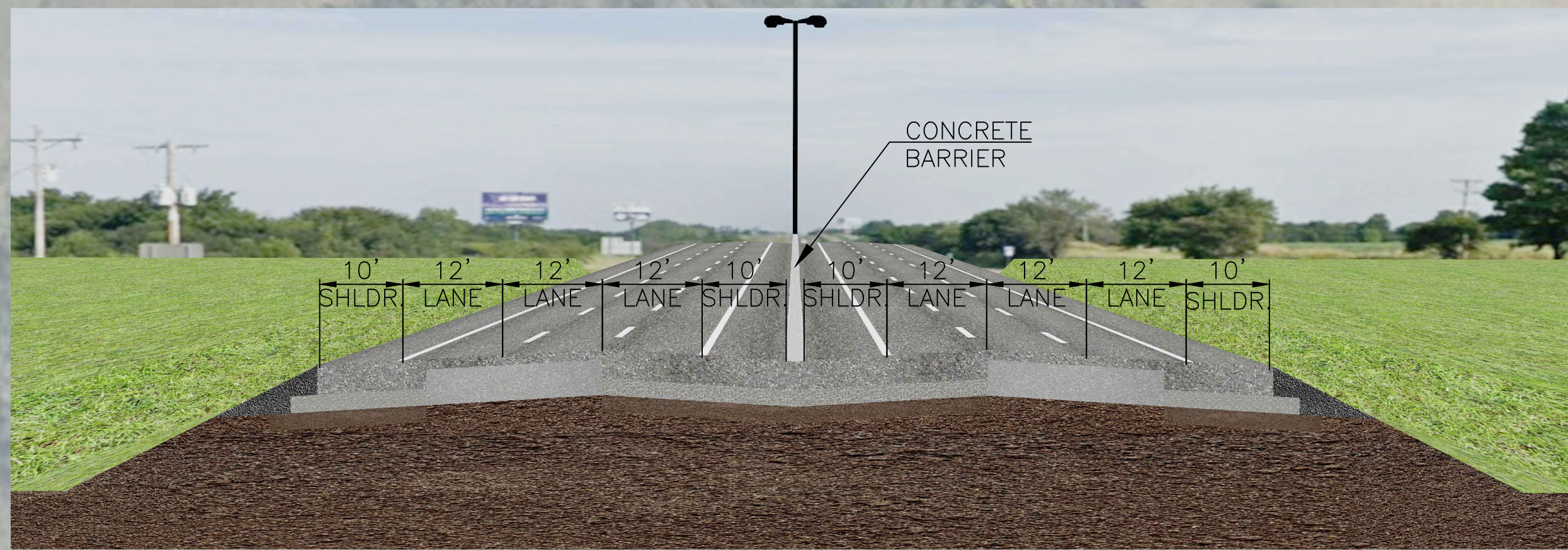
MAINLINE TYPICAL
