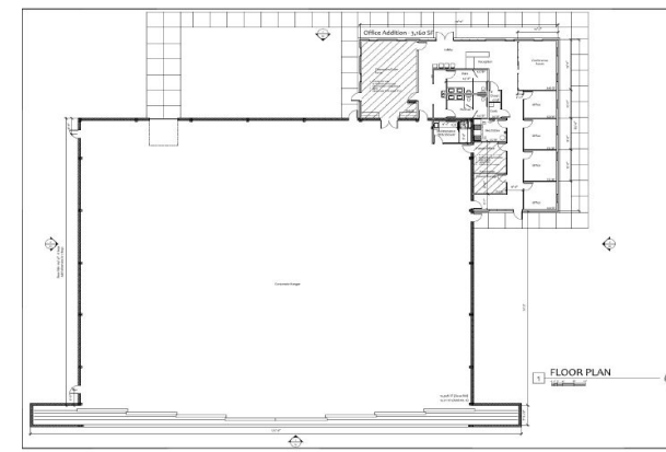
Corporate Hangar Floor Plan
