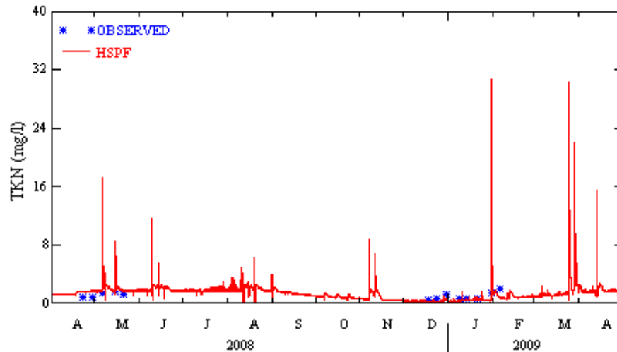
Figure A-30 Comparison of observed and simulated stream TP concentrations at Elm station
