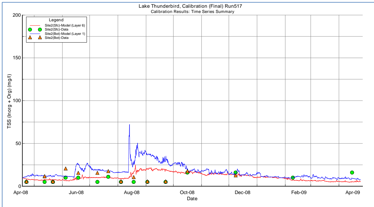
Figure B-85 TS_Cal011_TSS(io)_Site2 (Surface & Bottom)
