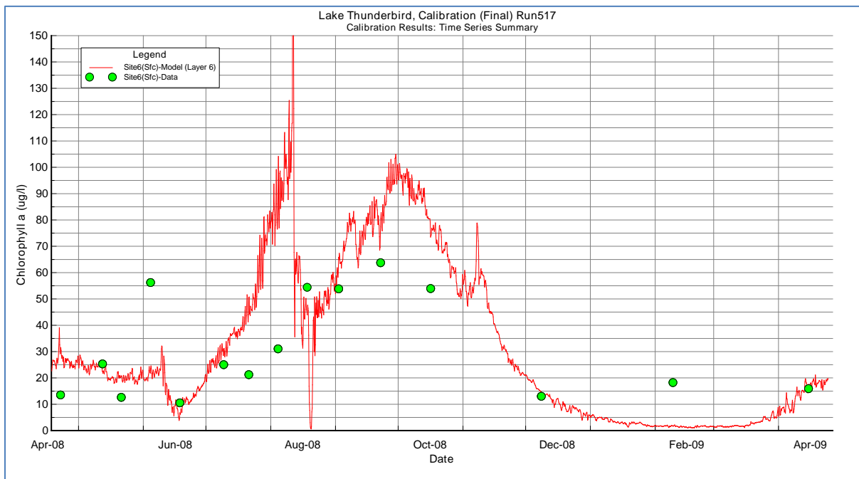
Figure B-91 TS_Cal031_Ch1-a_Site6 (Surface)
