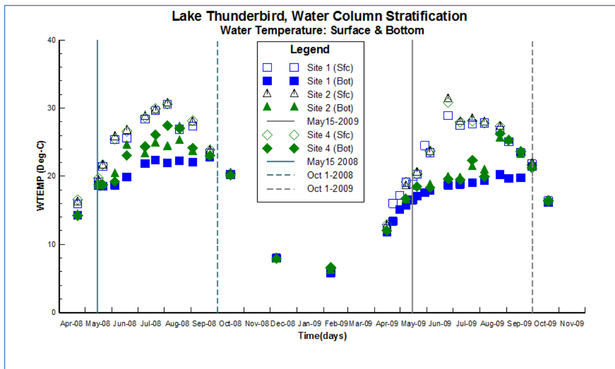
Figure 4-5 Surface and Bottom Layer Water Temperature for Lacustrine Sites in Lake Thunderbird, 2008 - 2009.
