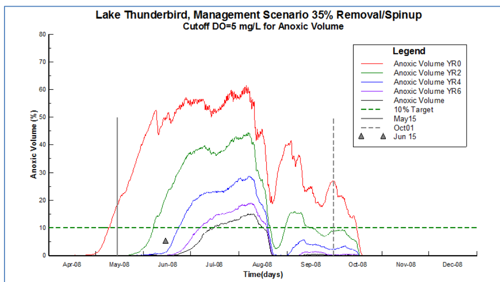
Figure 4-11 Whole Lake Volume Weighted Percentage of Lake Less than Cutoff Concentration of 5 mg/L for Spin-Up Years (Year 0, Year 2, Year 4, Year 6, and Year 8)
