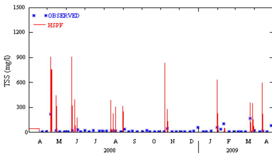
Figure A-19 Comparison of observed and simulated stream TSS concentrations at L17station
