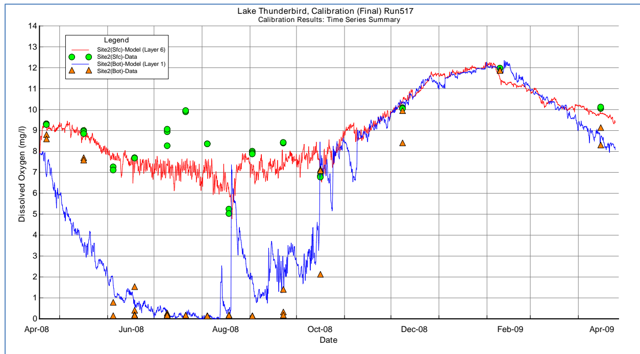
Figure B-39 Model-Data Comparison of Dissolved Oxygen for Surface Layer (k=6) and Bottom Layer (k=1) for Site 2
