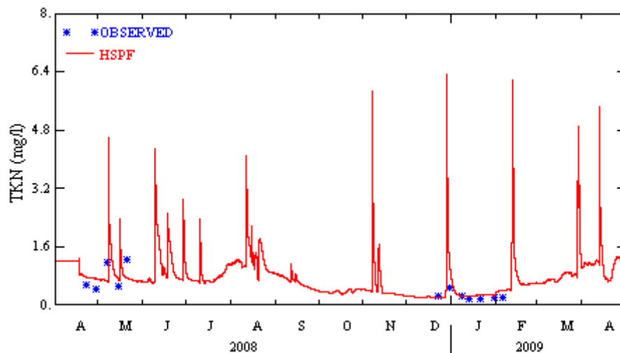
Figure A-28 Comparison of observed and simulated stream TKN concentrations at Hog station
