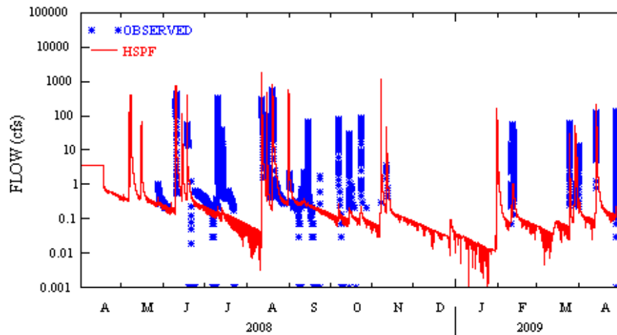
Figure A-109 Comparison of observed and simulated stream flows at L60 station
