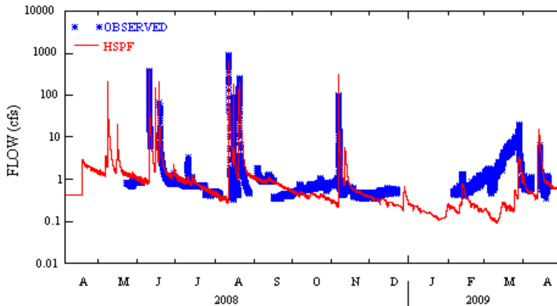
Figure A-8 Comparison of observed and simulated stream flows at Hog station
