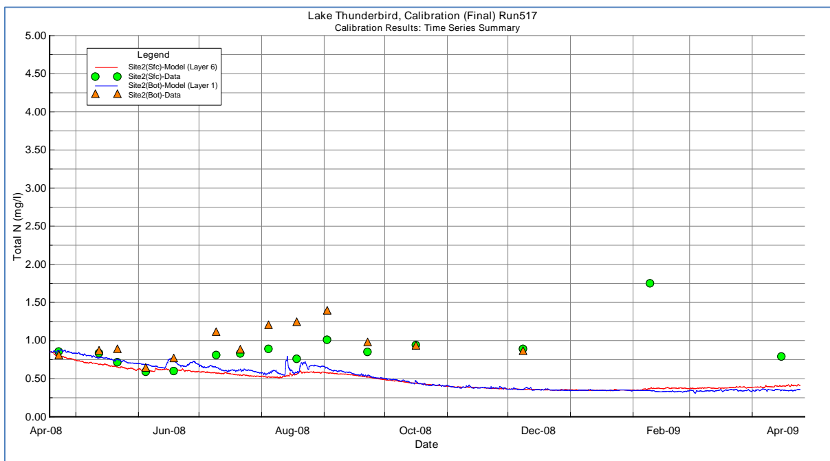
Figure B-92 TS_Cal035_Tot N_Site2 (Surface & Bottom)
