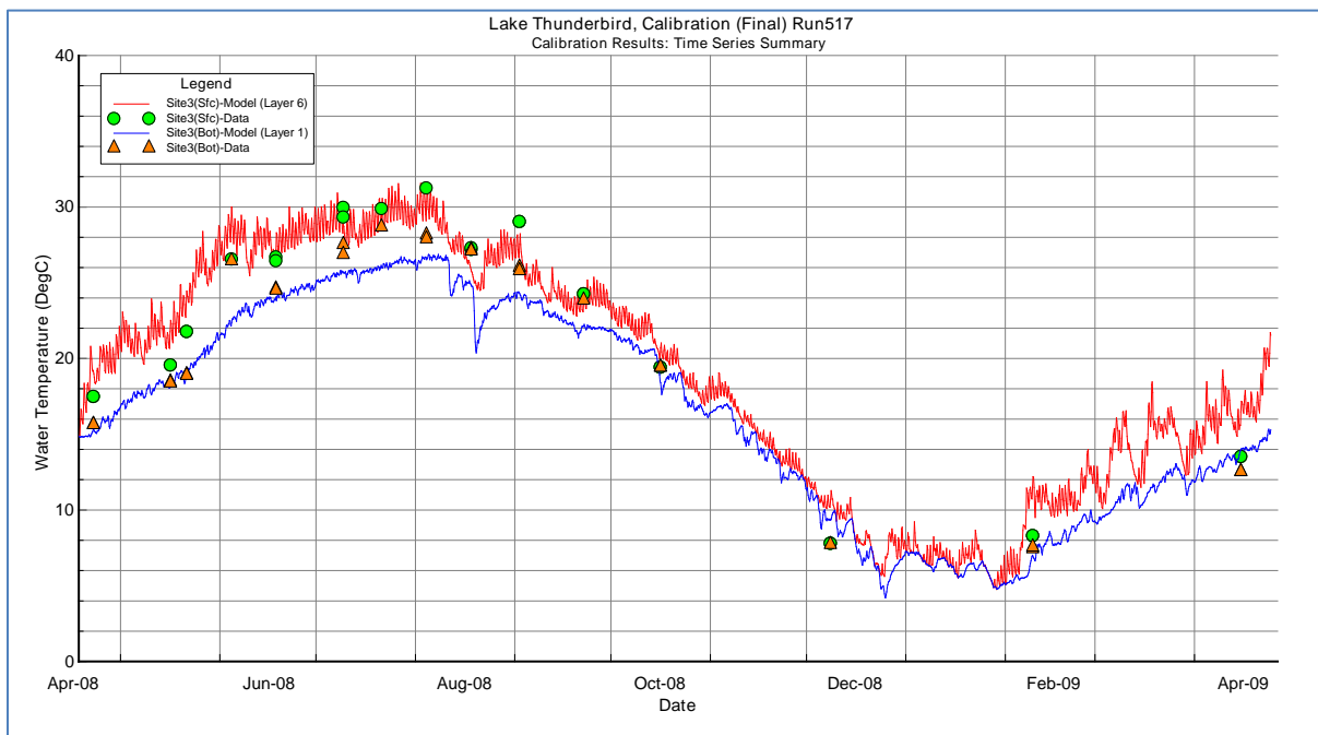
Figure B-83 TS_Cal004_Temp_Site3 (Surface & Bottom)
