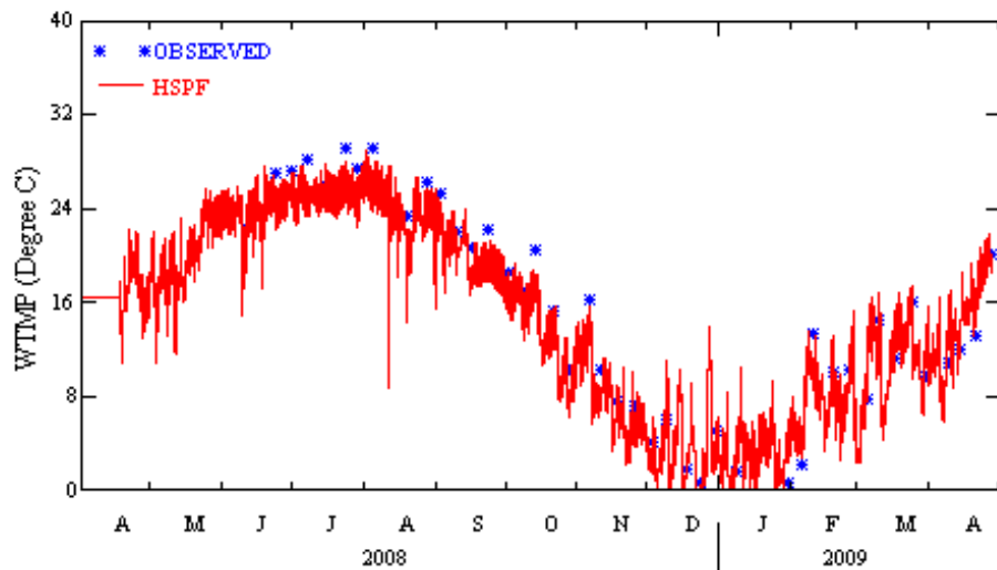
Figure A-16 Comparison of observed and simulated stream temperatures at Rock station
