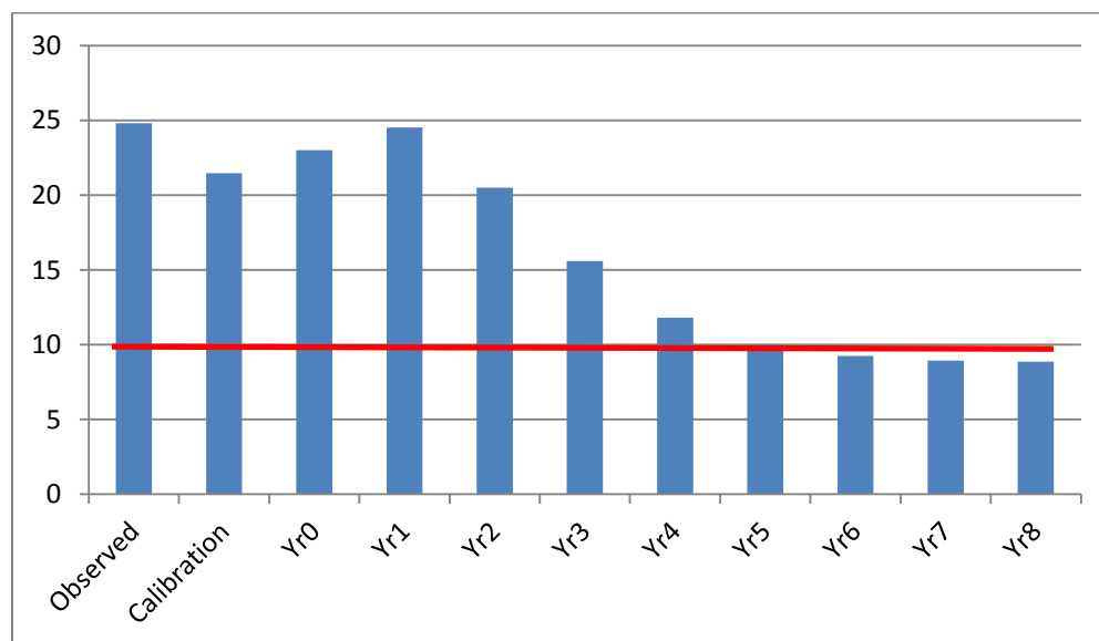
Figure 4-3 Surface chlorophyll-a (µg/L): Spin-Up Model Results for 35% Removal and Annual Average of all Eight Sites
