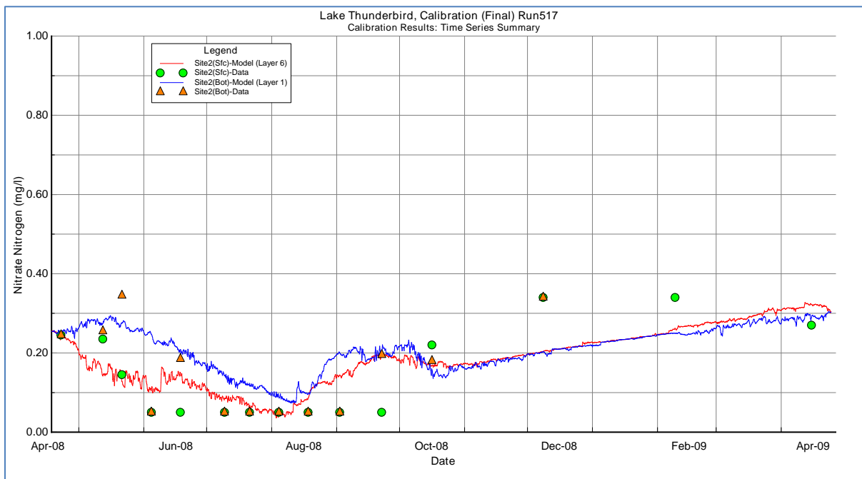
Figure B-100 TS_Cal067_NO3-N_Site2 (Surface & Bottom)
