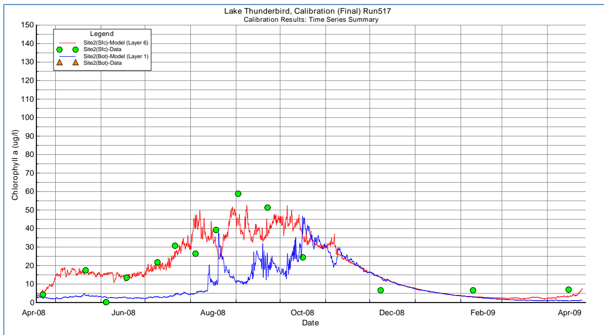
Figure B-43 Model-Data Comparison of Chlorophyll-a, Surface Layer (k=6) for Site 2.
