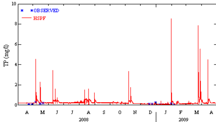
Figure A-32 Comparison of observed and simulated stream TP concentrations at L17 station
