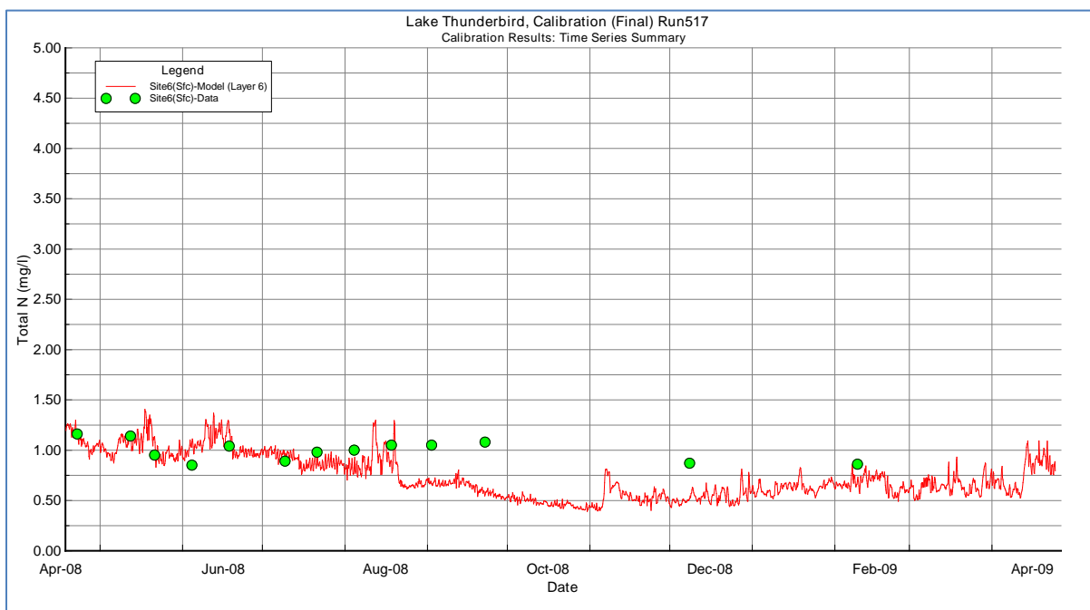
Figure B-93 TS_Cal039_Tot N_Site6 (Surface)
