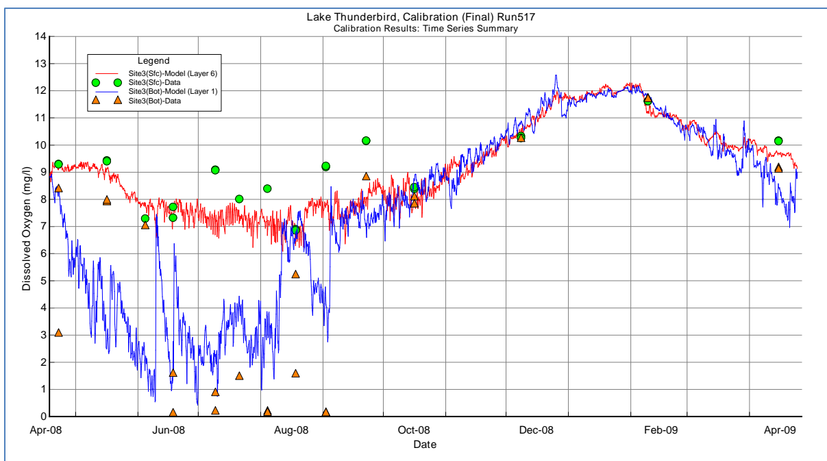
Figure B-88 TS_Cal020_DO_Site3 (Surface &amp; Bottom)
