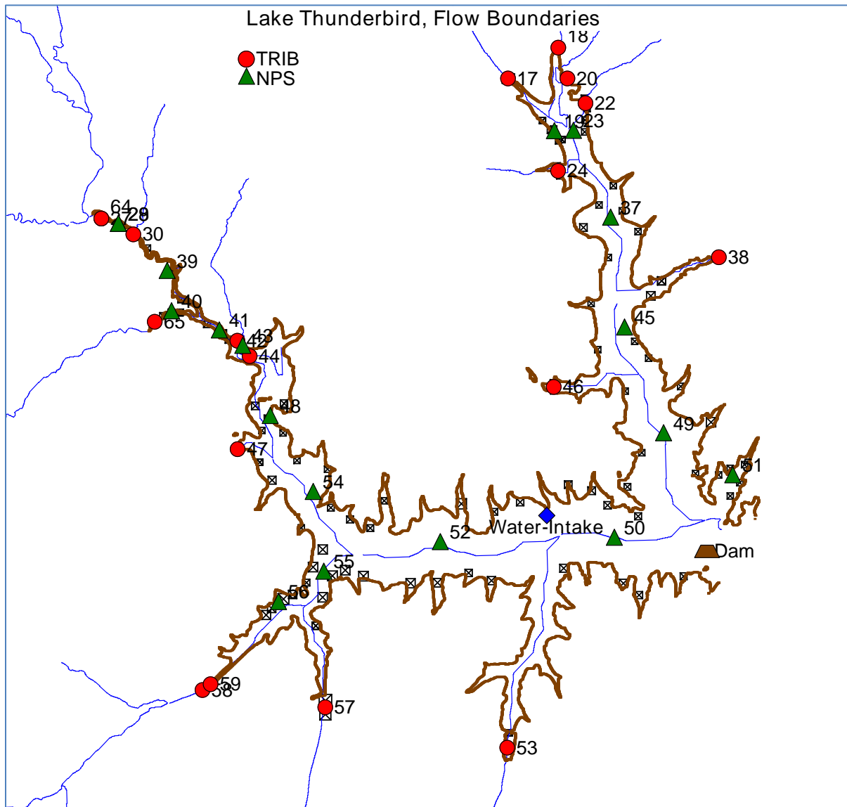
Figure B-33 Boundary Locations for HSPF tributary outlets and NPS distributed flow, Water Supply Intakes and Release at the Dam
