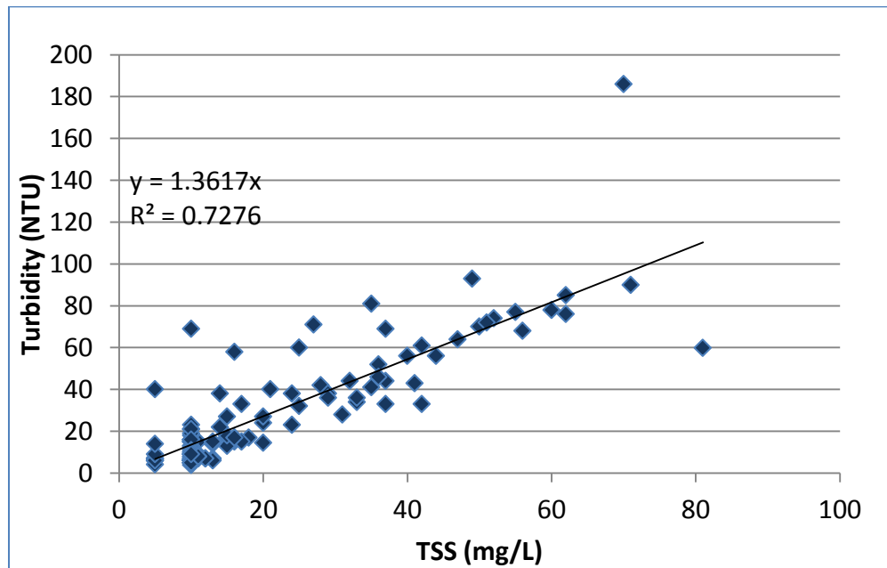
Figure B-37 TSS (mg/L) vs. Turbidity (NTU) Regression Relationship ( R^2=0.7276 ) for Lake Thunderbird
