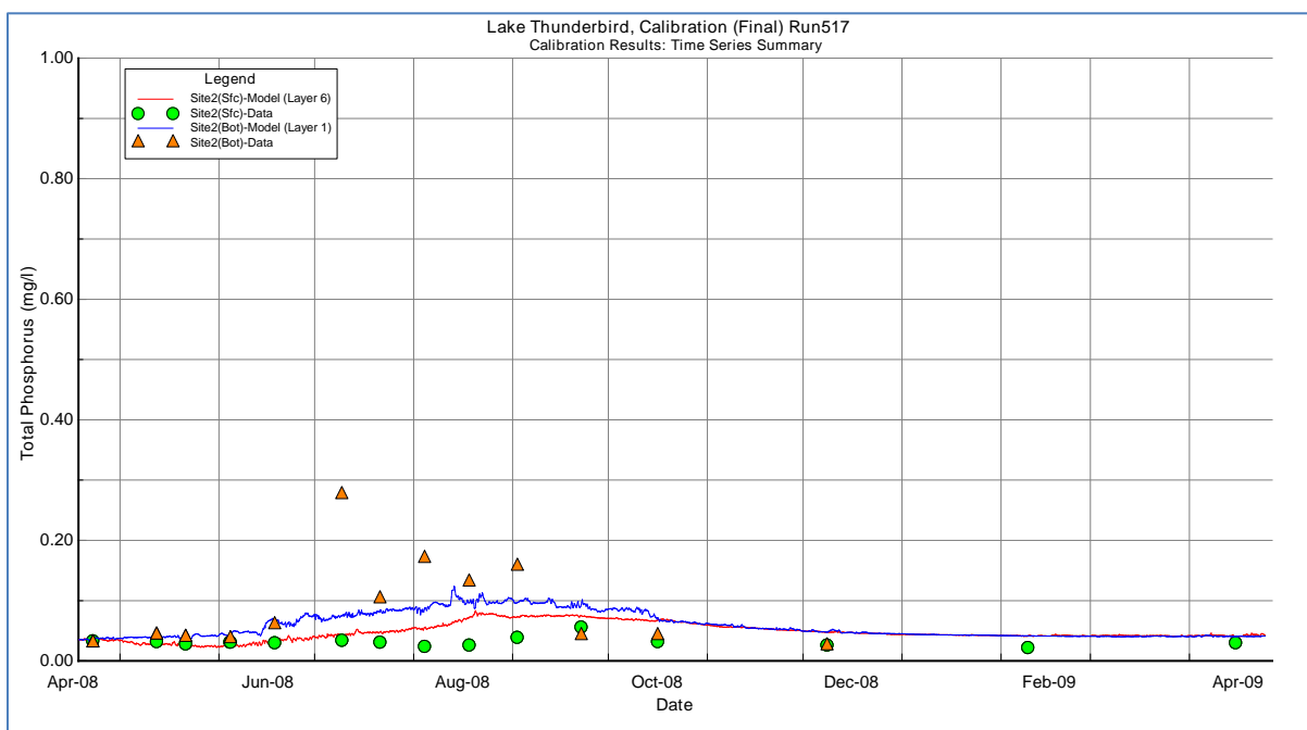
Figure B-94 TS_Cal043_Tot P_Site2 (Surface & Bottom)
