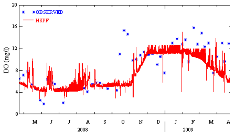
Figure A-254 Comparison of observed and simulated stream DO concentrations at L60 station
