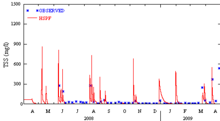
Figure A-21 Comparison of observed and simulated stream TSS concentrations at Rock station
