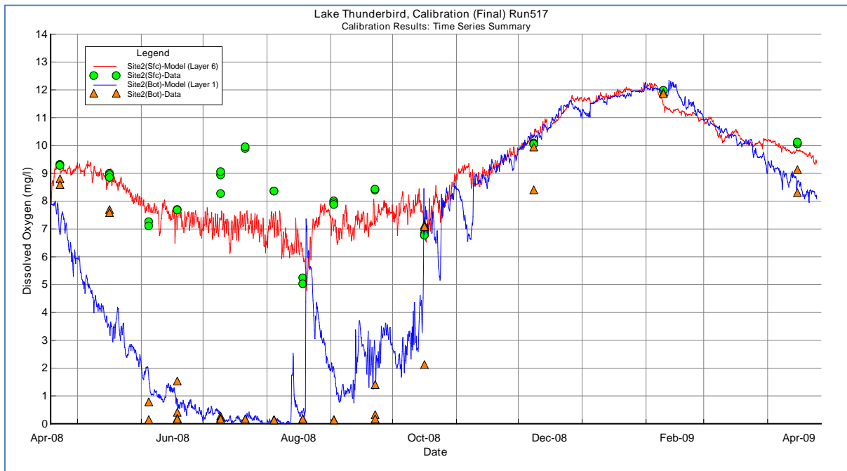
Figure B-87 TS_Cal019_DO_Site2 (Surface &amp; Bottom)
