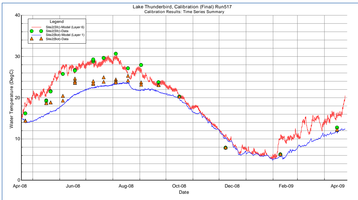
Figure B-82 TS_Cal003_Temp_Site2 (Surface & Bottom)
