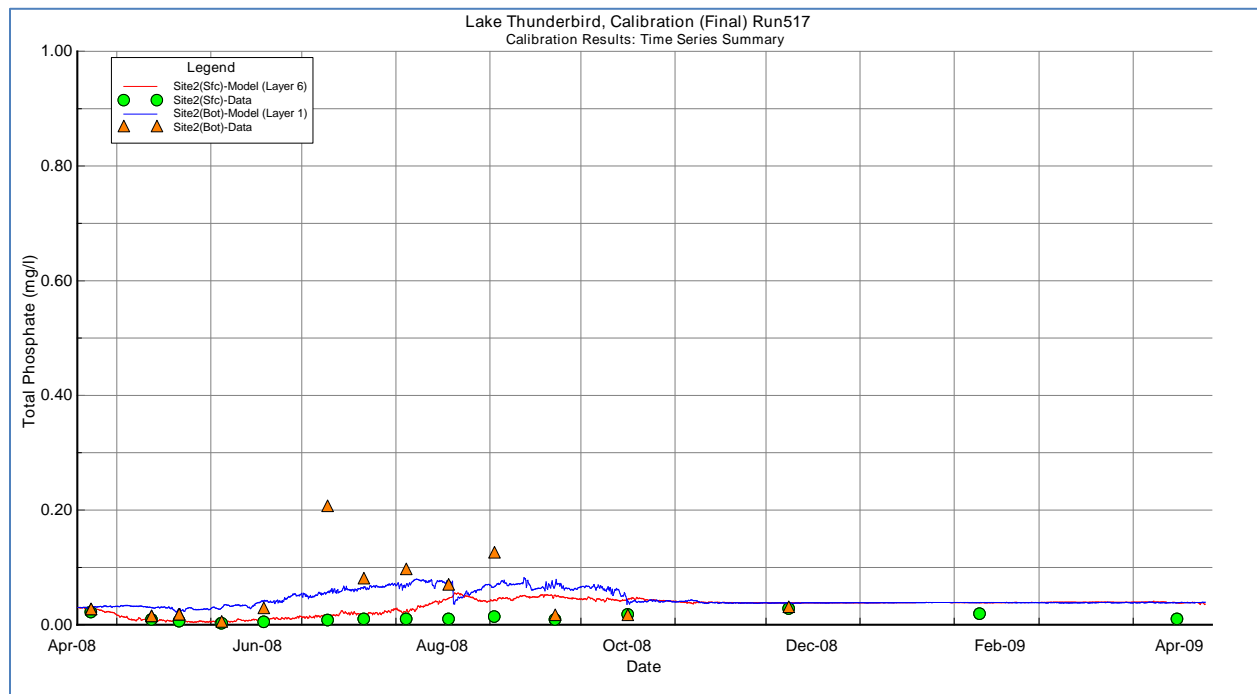
Figure B-45 Model-Data Comparison of Total-Phosphate-P (TPO4) for Surface Layer (k=6) and Bottom Layer (k=1) for Site 2.
