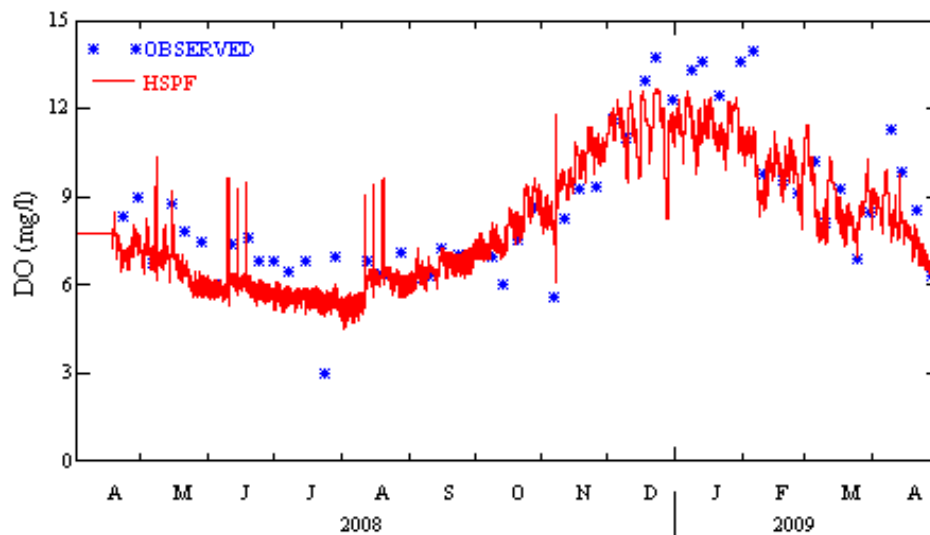
Figure A-22 Comparison of observed and simulated stream DO concentrations at Elm station
