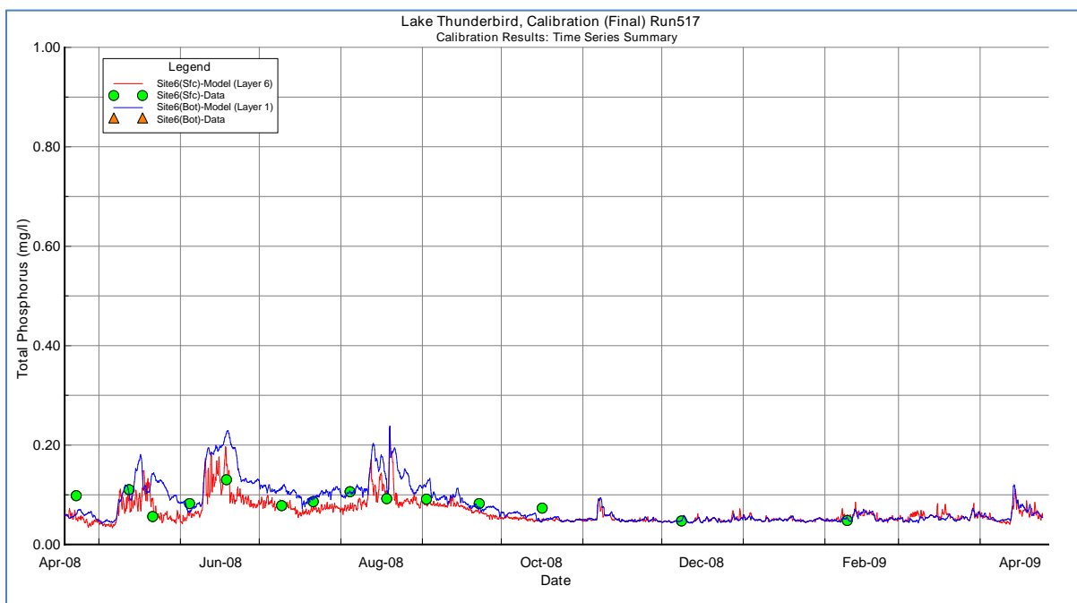
Figure B-95 TS_Cal047_Tot P_Site6 (Surface)
