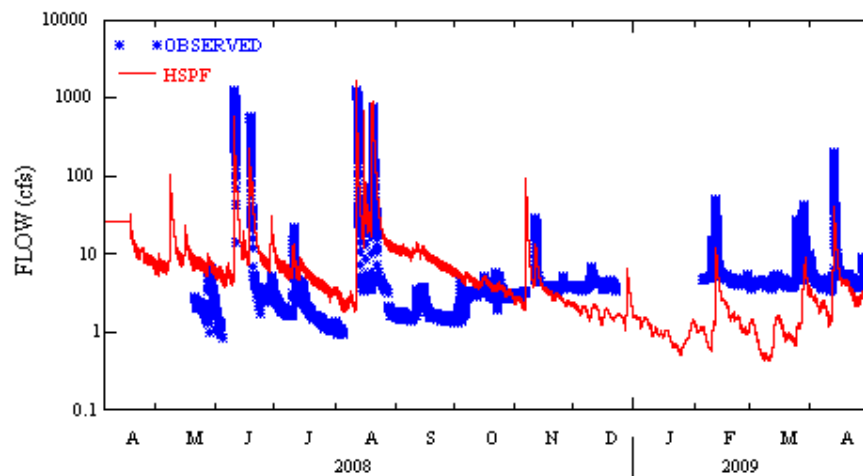
Figure A-9 Comparison of observed and simulated stream flows at L17 station
