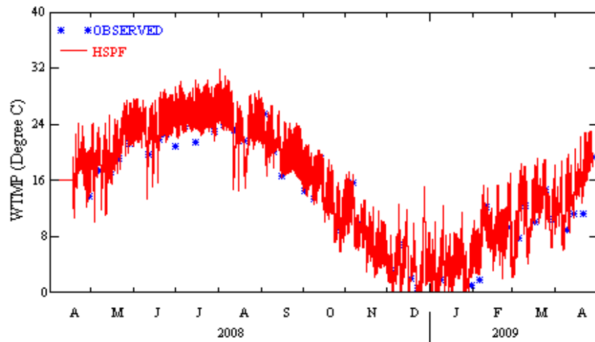
Figure A-13 Comparison of observed and simulated stream temperatures at Hog station
