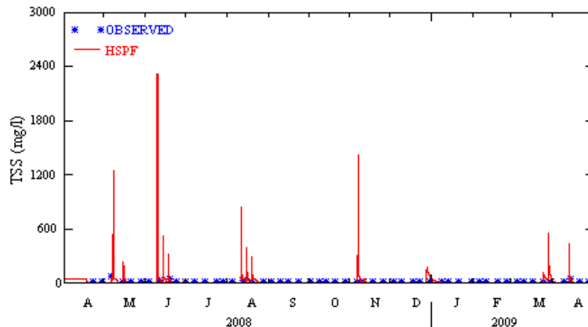
Figure A-18 Comparison of observed and simulated stream TSS concentrations at Hog station
