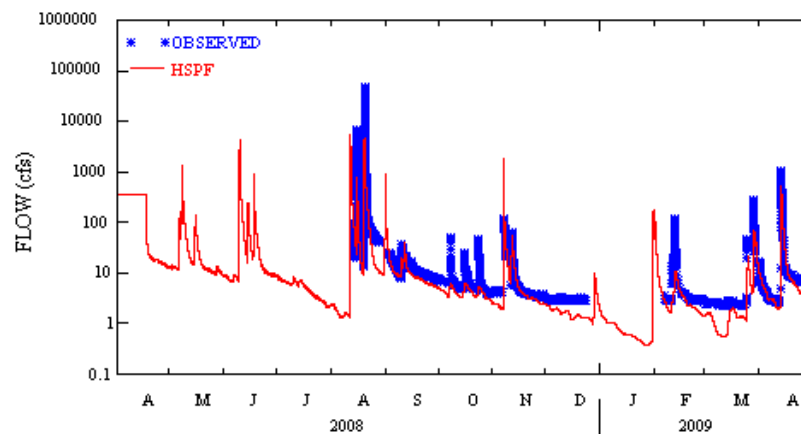
Figure A-11 Comparison of observed and simulated stream flows at Rock station
