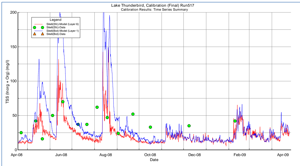
Figure B-86 TS_Cal015_TSS(io)_Site6 (Surface)
