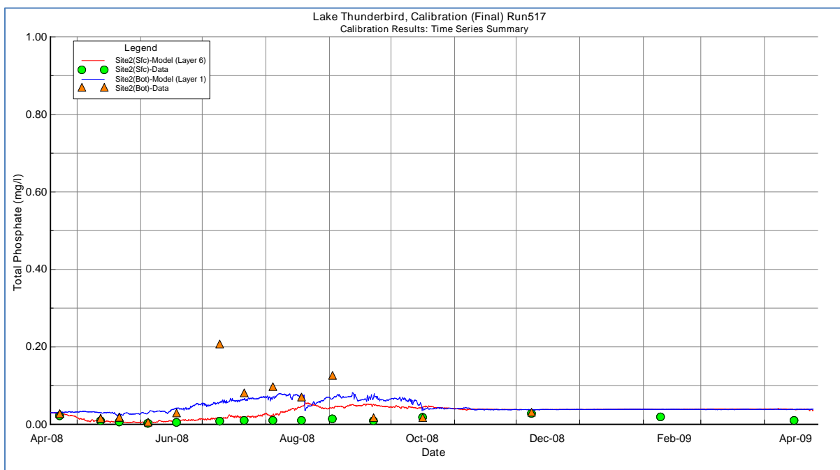
Figure B-96 TS_Cal051_TPO4-P_Site2 (Surface & Bottom)
