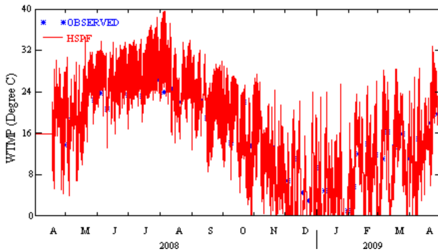
Figure A-15 Comparison of observed and simulated stream temperatures at L60 station
