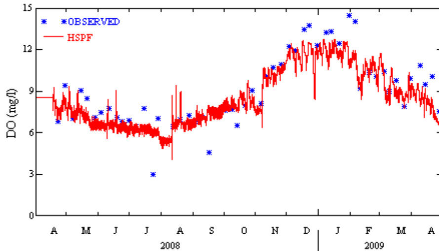
Figure A-24 Comparison of observed and simulated stream DO concentrations at L17 station
