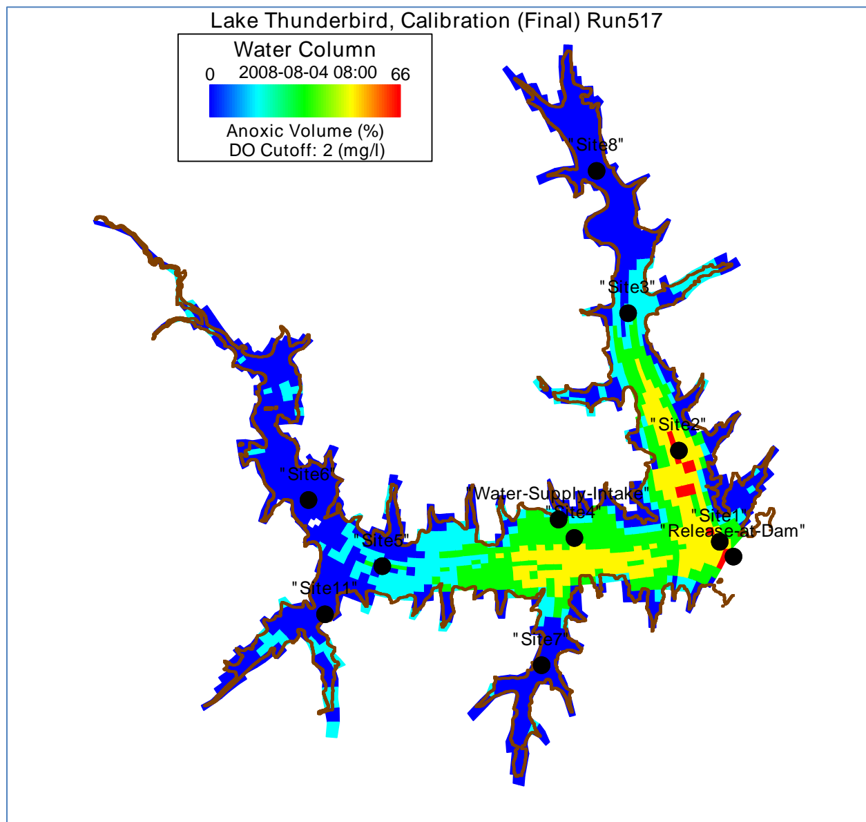
Figure B-40 Anoxic Volume of Lake Thunderbird on August 4, 2008 at 08:00 Color gradient for 6-layer model as follows for anoxic volume percentage: dark blue=0%; light blue=16%; green=33%; yellow=50% and red =66%
