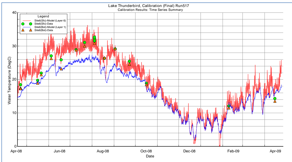
Figure B-84 TS_Cal007_Temp_Site6 (Surface & Bottom)
