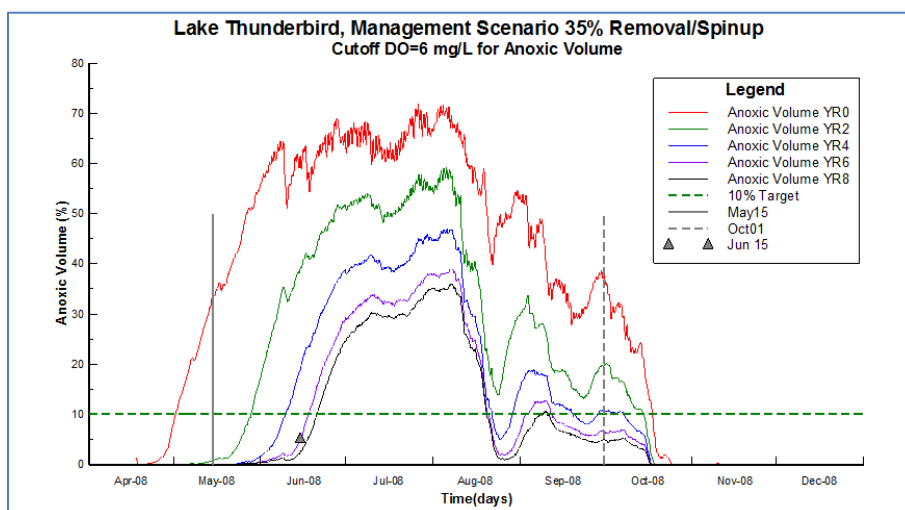
Figure 4-10 Whole Lake Volume Weighted Percentage of Lake Less than Cutoff Concentration of 6 mg/L for Spin-Up Years (Year 0, Year 2, Year 4, Year 6, and Year 8).
