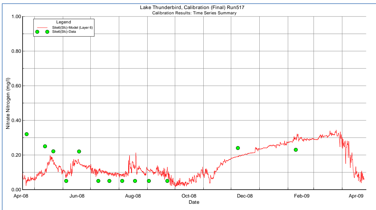
Figure B-101 TS_Cal071_NO3-N_Site6 (Surface)
