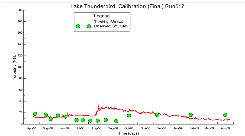
Figure B-38 Model-Data Comparison of Turbidity for Surface Layer (k=6) for Site 2
