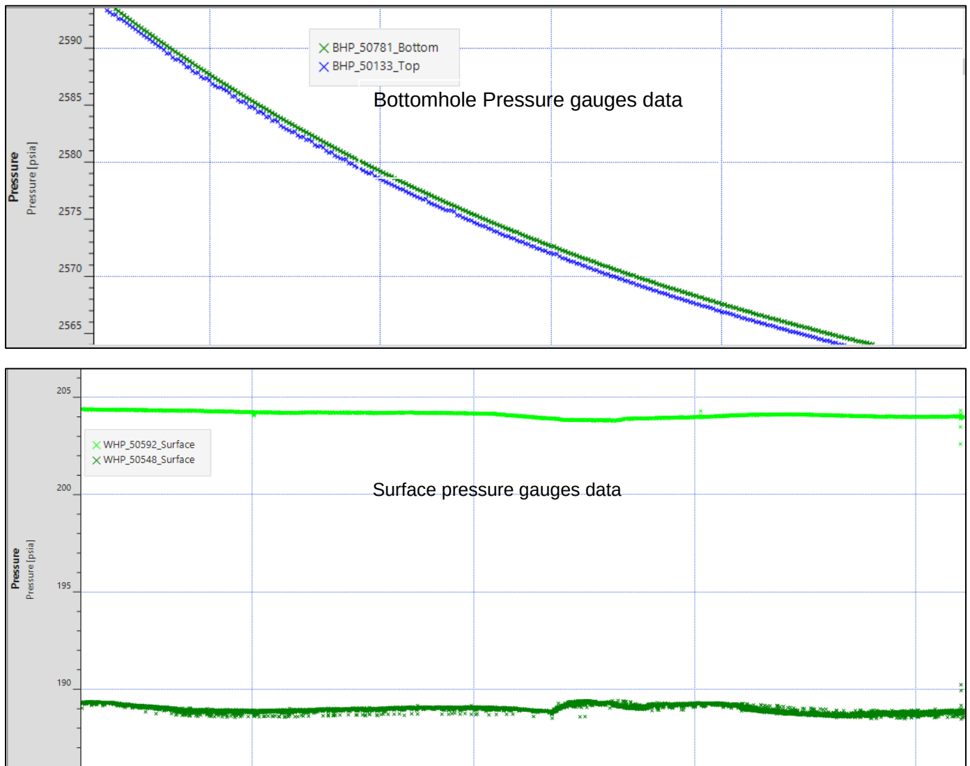
Figure 4: Bottom hole and surface pressure gauges data quality
