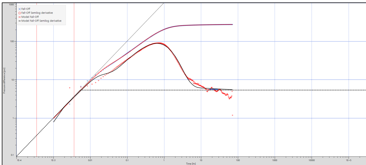
Figure 6: Log-Log Plot and PTA Model for pressure falloff with downhole gauge 50781 (Vertical Homogeneous Infinite)
