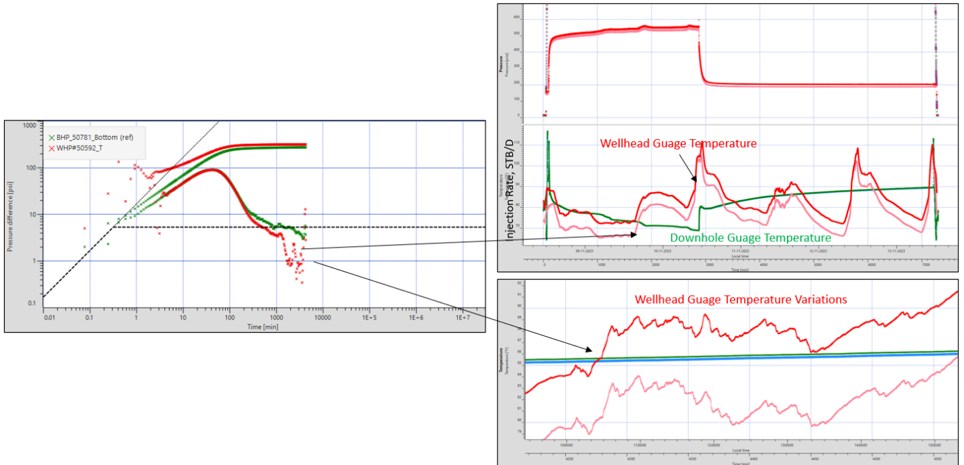
Figure 5: Early and late time pressure transient wellbore dynamics effect
