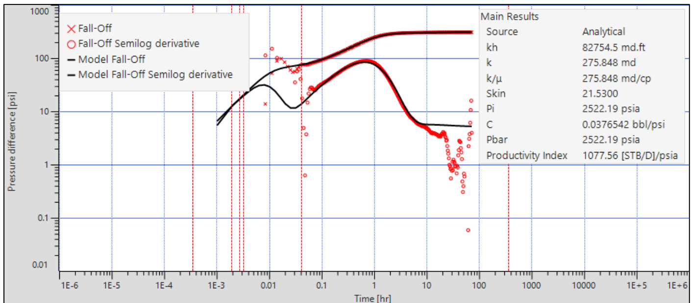
Figure 9: Log-Log Plot and PTA Model for pressure falloff with wellhead pressure gauge 50592 Transform (Vertical Homogeneous Infinite)
