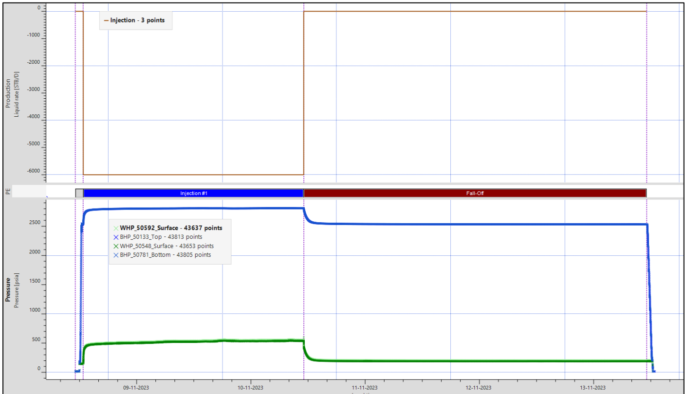
Figure 1: Cartesian Plot for Injection flow rate and Pressure Falloff for gauges #50133 and 50781 @ 5,340 ft and well head gauges #50548 and #50592 (WHP: green color, BHP: blue color, Injection rate: Brown color)
