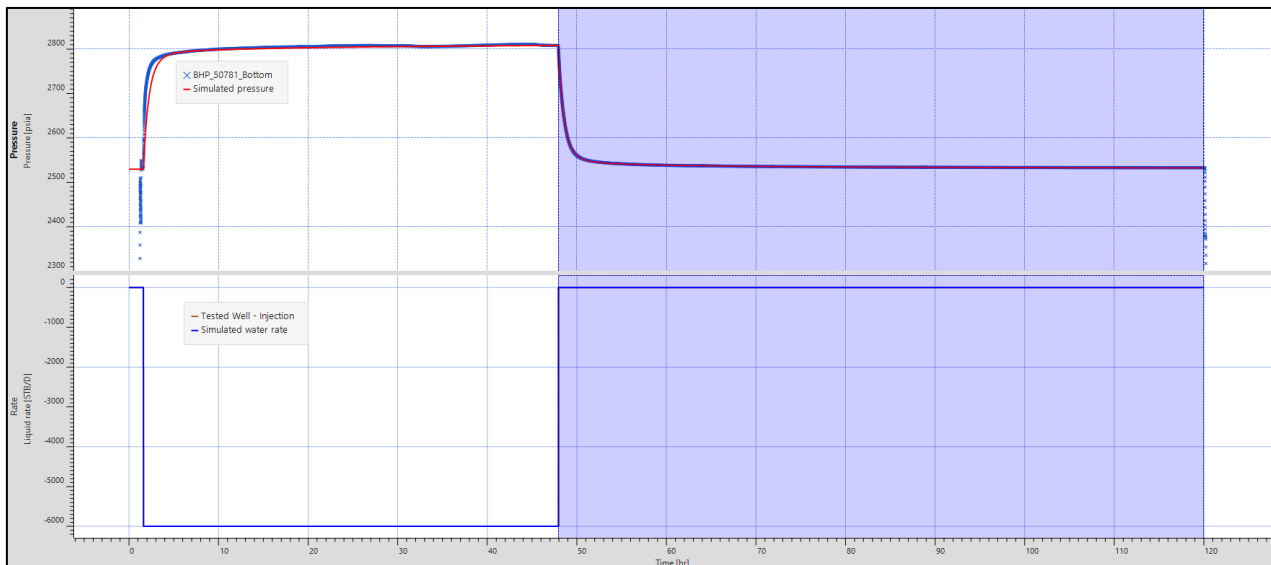
Figure 8: Top plot: Test bottomhole pressure data (blue color) and history match model (red), gauge 50781. Bottom plot: injection rate (STB/D).
