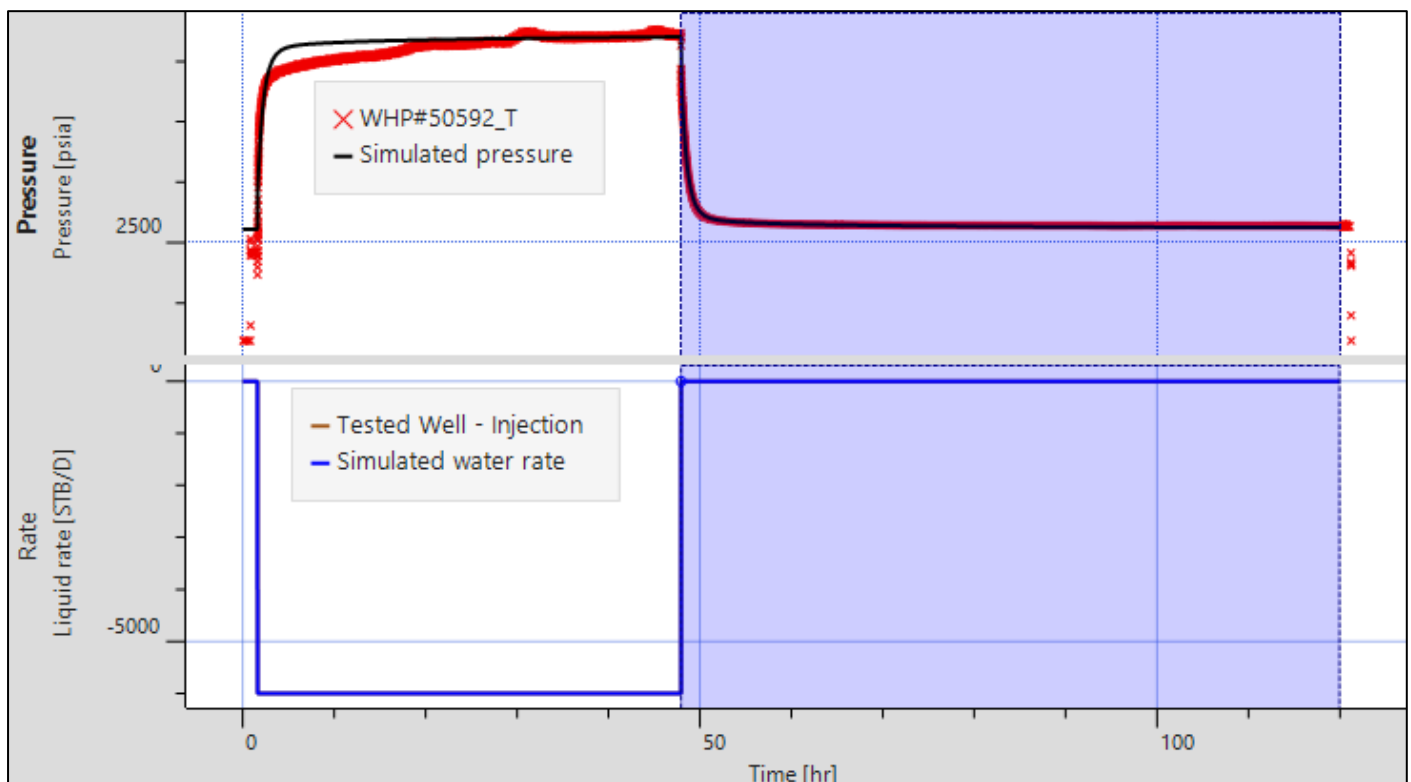
Figure 11. Test bottomhole pressure data (red color) and history match model (black), gauge 50592 (Wellhead gauge data Transform). Bottom plot: injection rate (STB/D).
