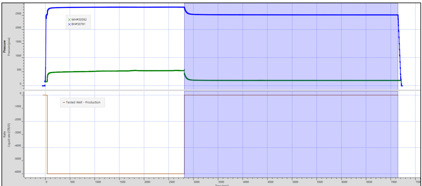
Figure 2: Pressure data for gauges considered for PTA analysis. Gauges #50781(bottom @ 5,340 ft in blue color and 50592 at well head in lime green color)
