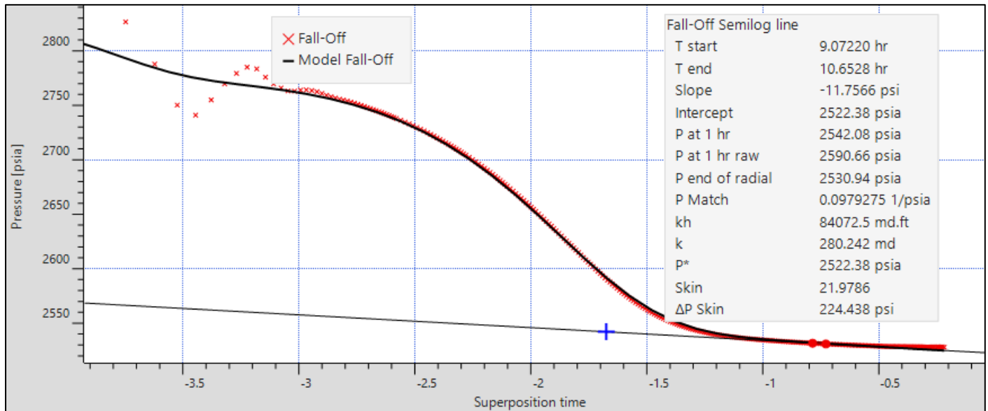
Figure 10. Semi-log Diagnostic Plot and model for Pressure Falloff with downhole gauge 50592.
