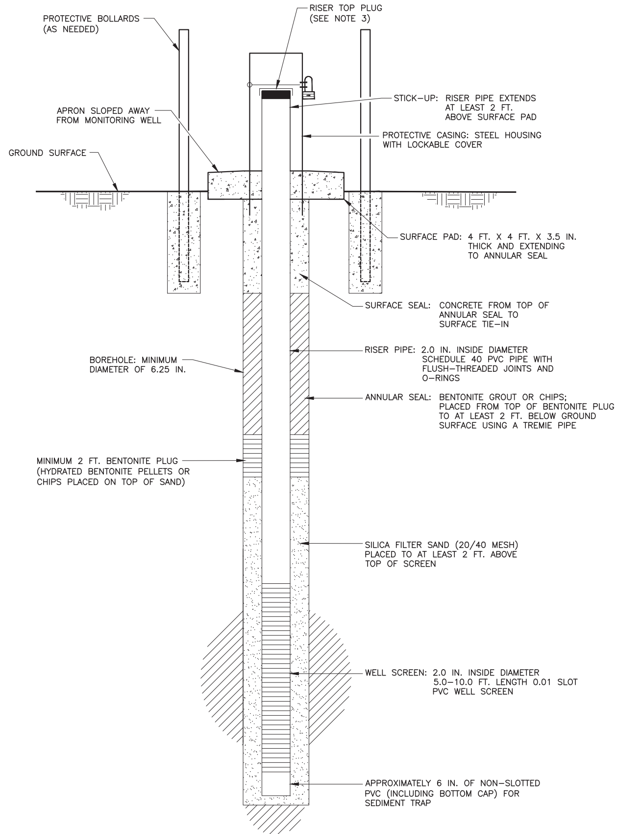
TYPICAL MONITORING WELL DETAIL NOT TO SCALE
