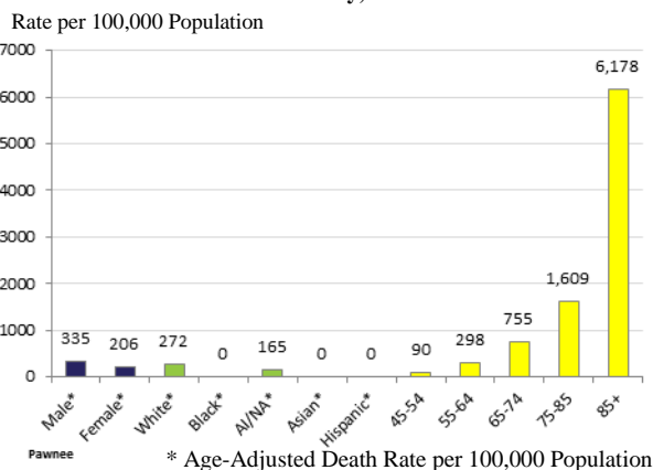
Heart Disease Death Rates by Demographic Groups, Pawnee County, 2008-2012
